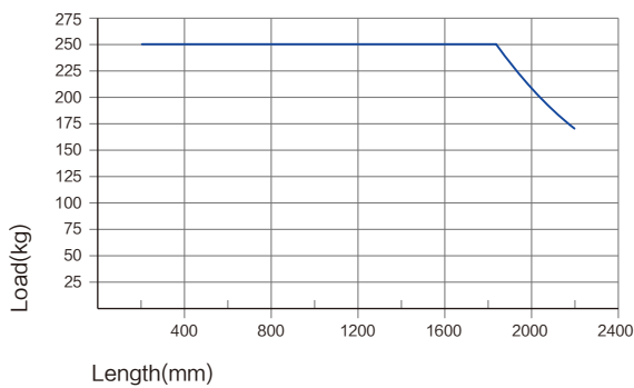
■ Tube \Phi 80 \times 3.0 , shaft \Phi 20 , internal thread
