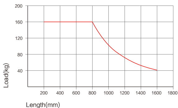
■ Tube \Phi 50 \times 1.5 , shaft \Phi 12/15 , internal thread
