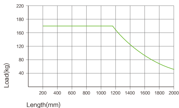
■ Tube \Phi 60 \times 2.0 , shaft \Phi 12/15 , internal thread
